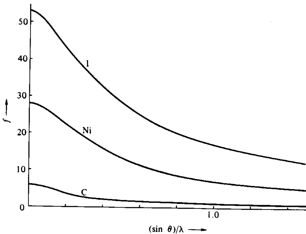
Fig. 4-8 Atomic form factors for representative atoms: iodine, nickel, and carbon.
