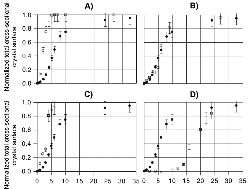
Fig. 4 Exemplary time-courses of the normalized total cross-sectional crystal surface of sitting-drops using ethanolammonium formate (IL1.1). c_{\text{Lysozyme}} = 50 \text{ g l}^{-1} , c_{\text{NaCl}} = 25 \text{ g l}^{-1} , 50 mM acetate buffer, pH = 6.3–7.0. Two independent experiments for each concentration level of IL. The required time to
